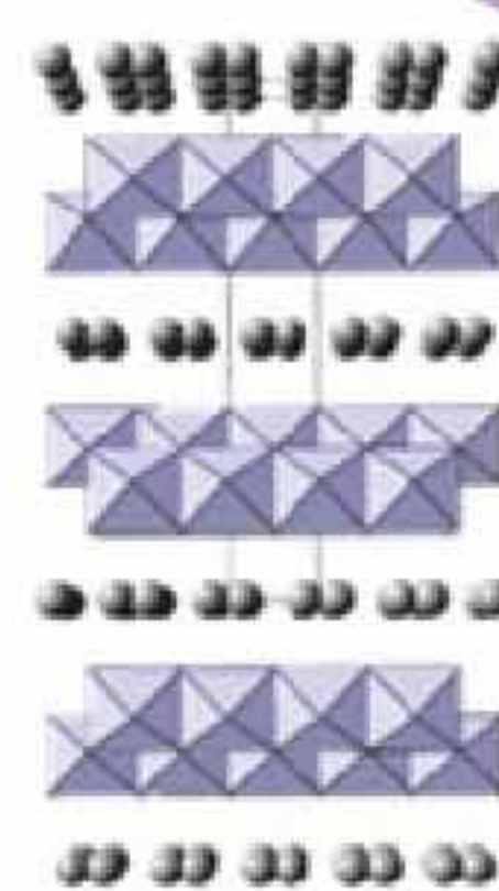
Layered titanate
