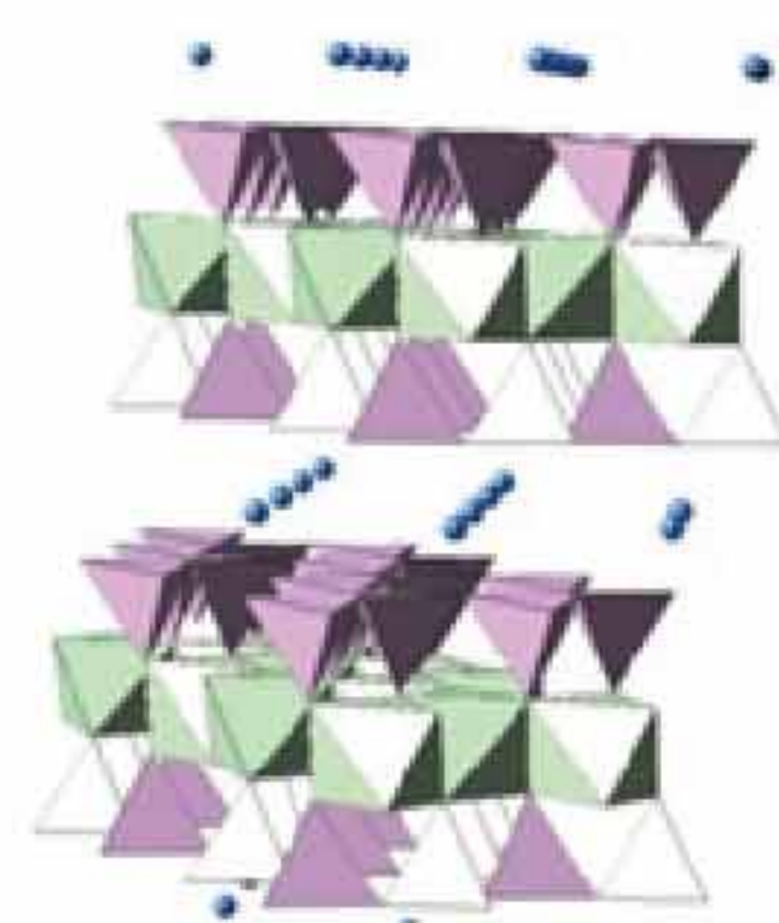
Clay
