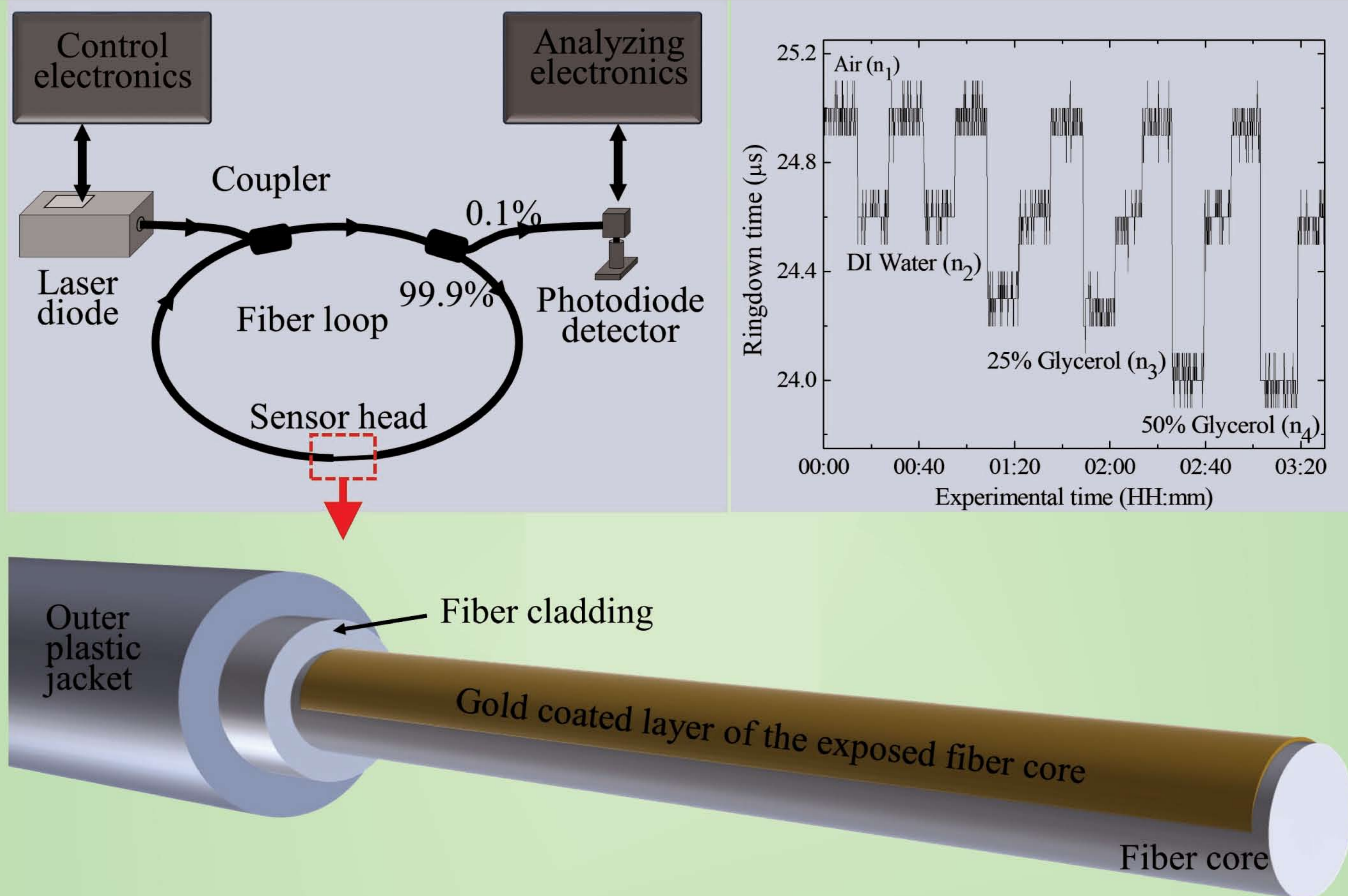
Surface plasmon-based fiber loop ringdown: system, sensor head, and sensor's response
